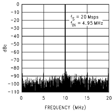
Spectral Response
