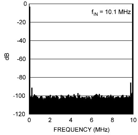
Spectral Response, 10.1 MHz Input
